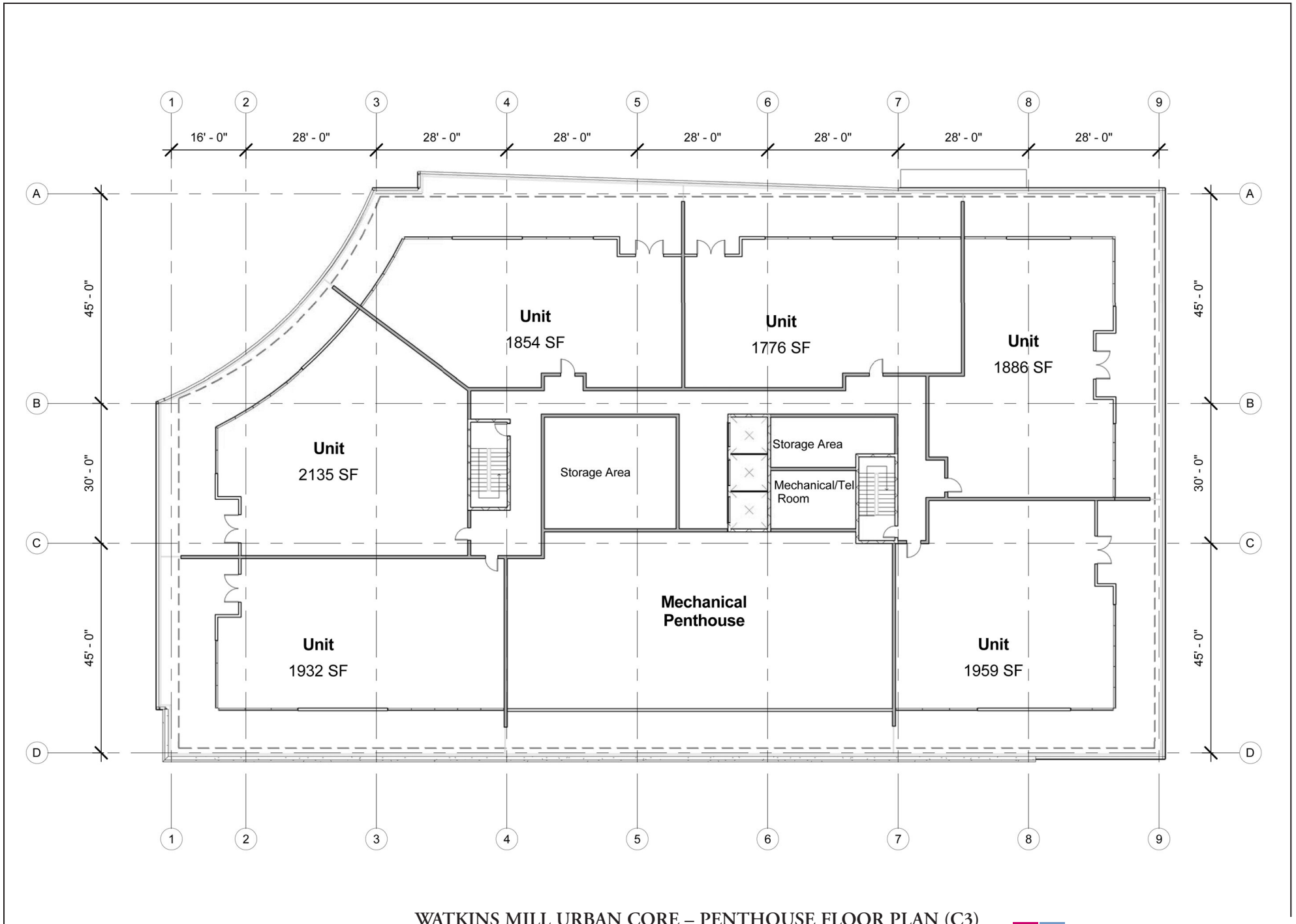
WATKINS MILL URBAN CORE – PENTHOUSE FLOOR PLAN (C3)
